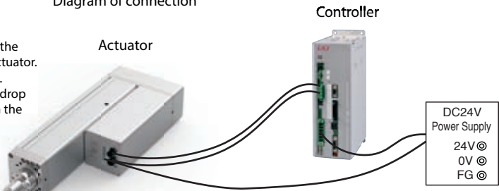
Diagram of connection
