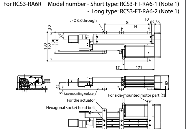
Foot Bracket Standard Mounting Position
