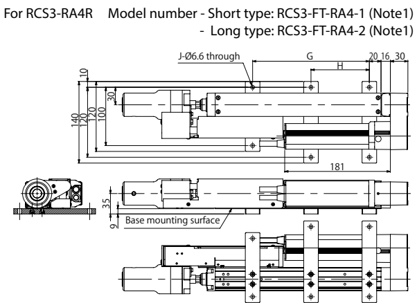
Foot Bracket Standard Mounting Position
